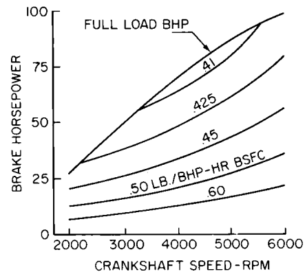
Fig. 15 SCORE 70 series 1007R estimated part load performance.
