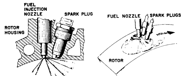
Fig. 3 shower head sc nozzle design.
