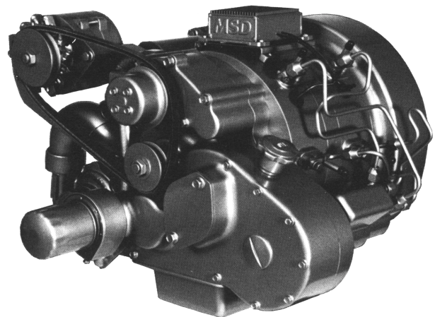
Fig. 11 mock-up of engine configuration resulting from value concepts study.
