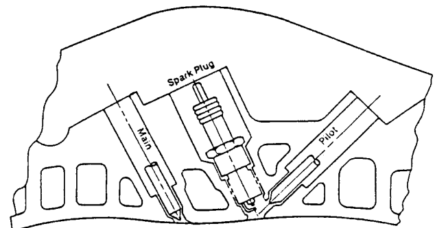
Fig. 4 dual nozzle stratified charged configuration.
