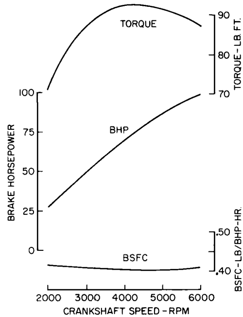
Fig. 14 SCORE 70 series 1007R estimated full load performance.
