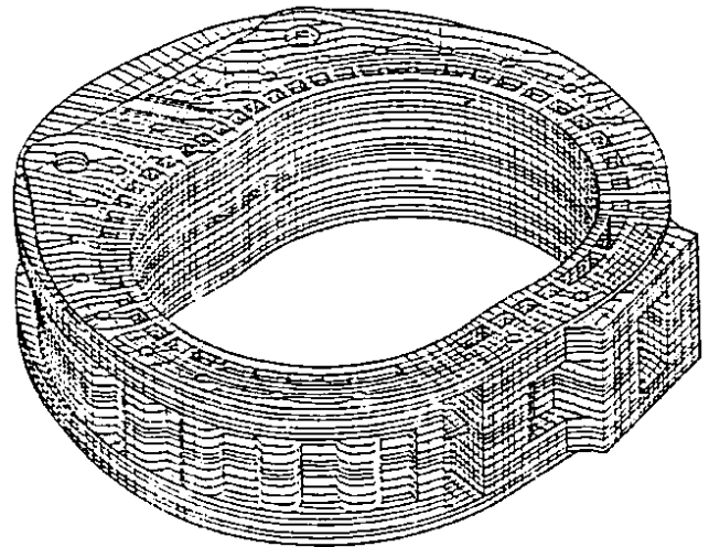
Fig. 8 FEM of rotor housing modified for turbocharging.
