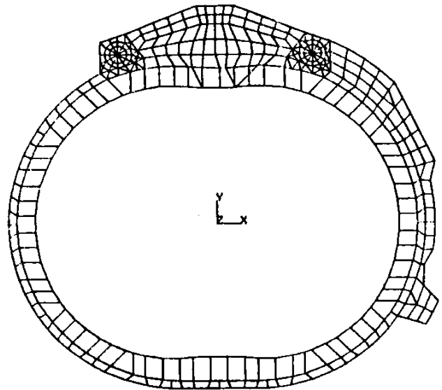
Fig. 7 naturally aspirated version of rotor housing.
