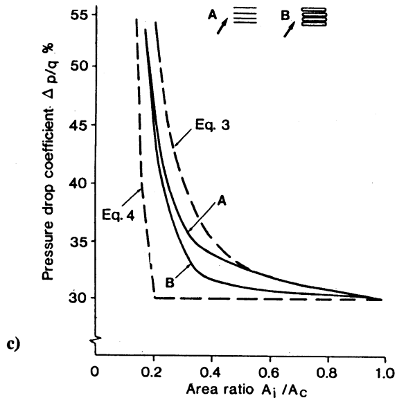
Fig. 9 Oblique flow effects: a) flow model, b) results from Ref. 2, and c) results from Ref. 15.
